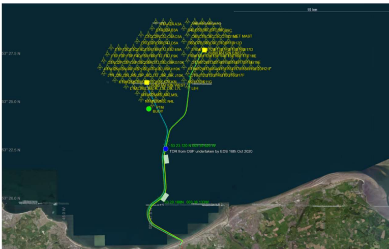
Figure 1 - Gwynt-Y-Mor site with suspected fault location shown
