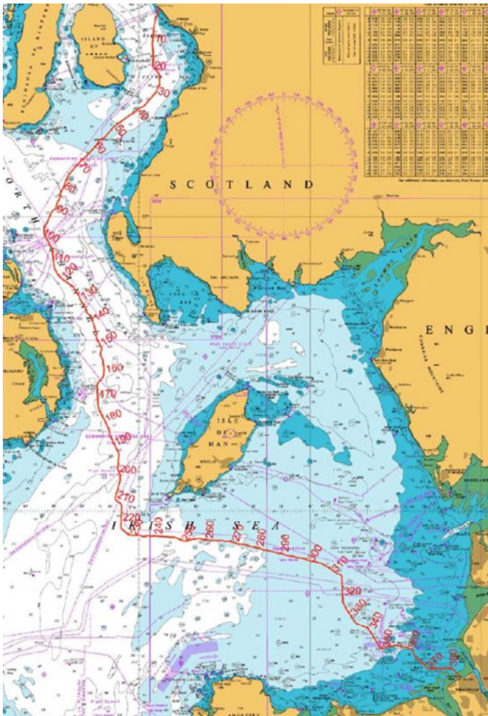
Figure 1: Survey Extents
