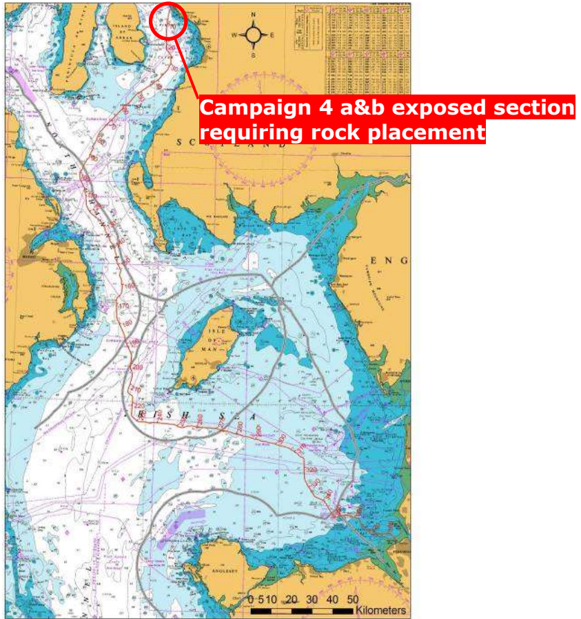
Figure 1 – Western Link cable route - Rock Placement Works Ardnail Bay
