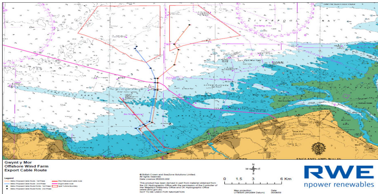
Admiralty Chart Layout of Gwynt y Mor including Export Cable Routes
