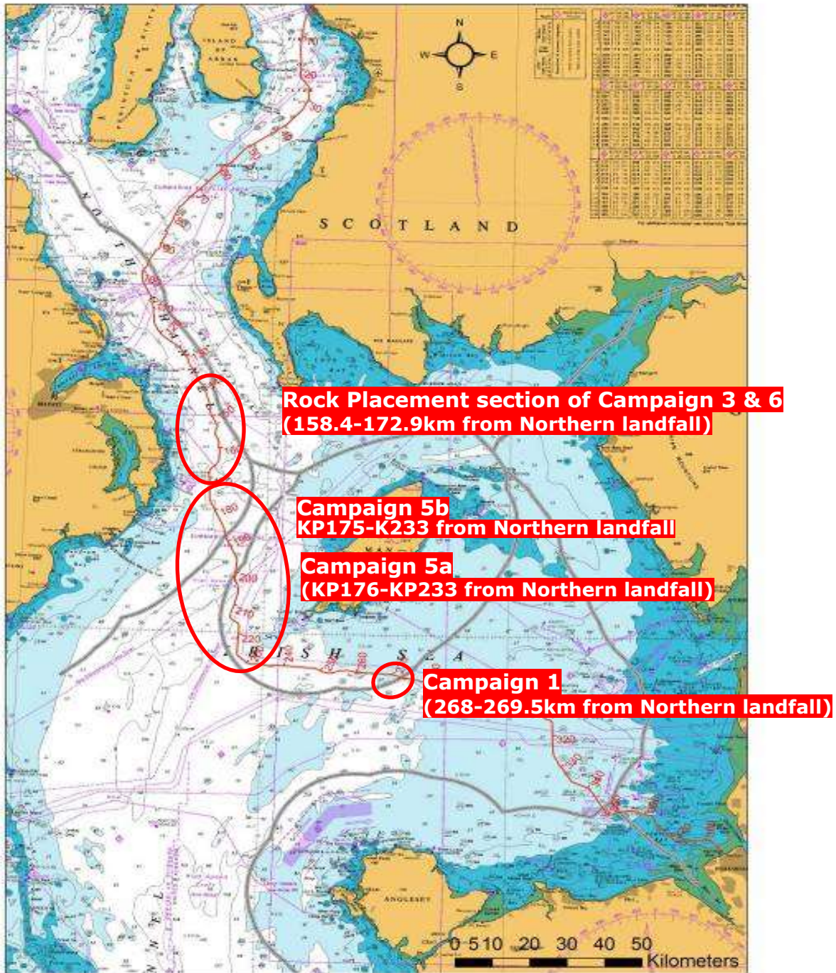
Figure 1 – Western Link cable route – Installation campaigns
