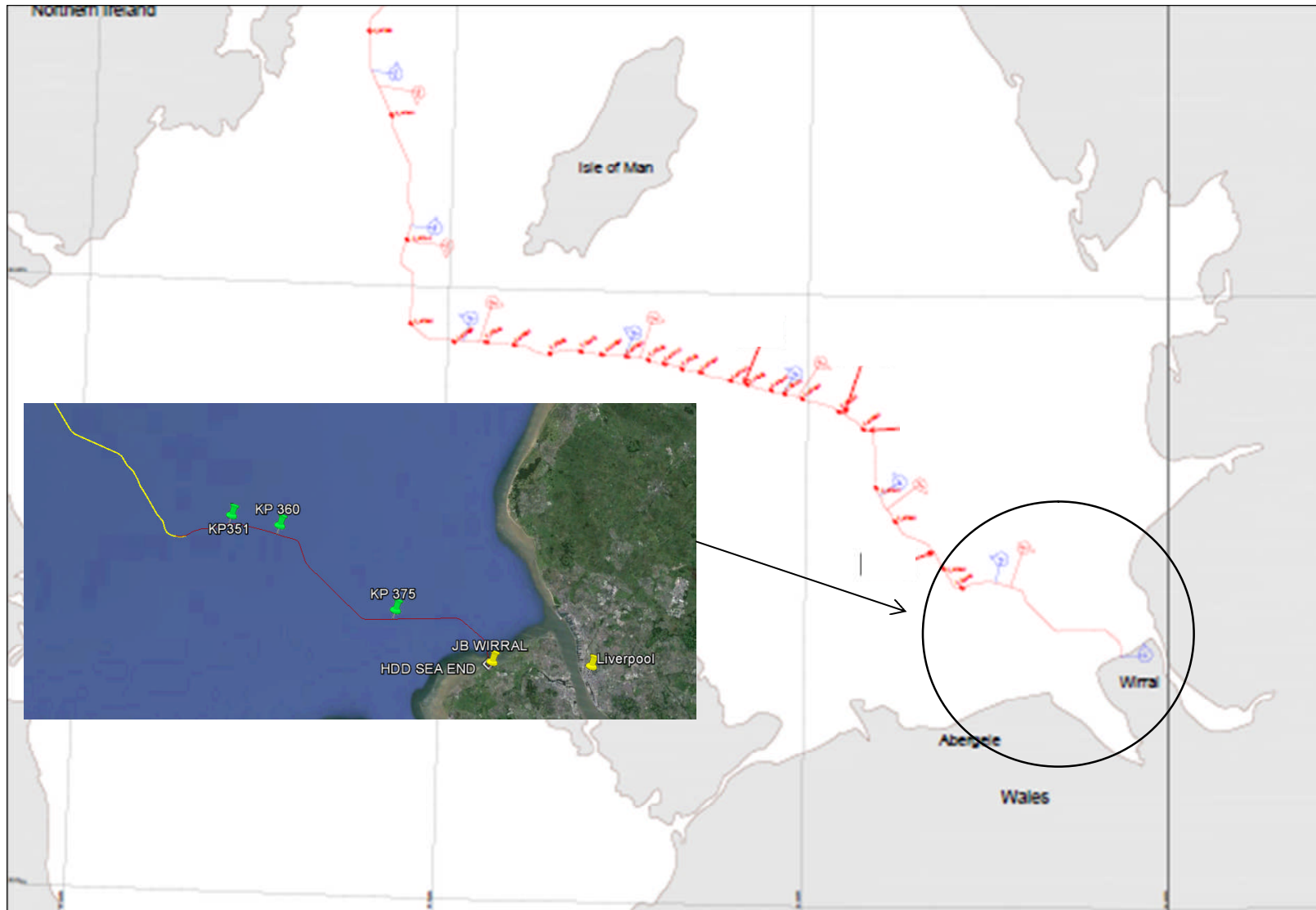
Figure 1 – Western Link cable route and Liverpool bay Shallow Water installation section
