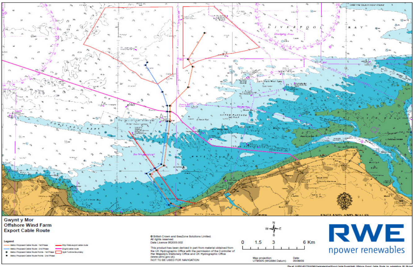
Admiralty Chart Layout of Gwynt y Môr including Export Cable Routes
