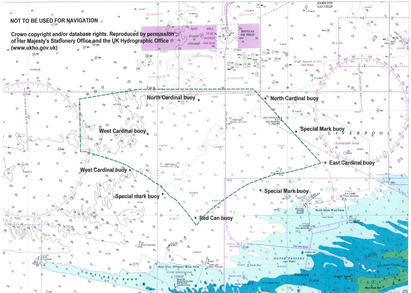
Navigation Buoy Layout at Gwynt y Mor Offshore Wind Farm
